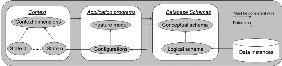
Fig. 1. DISA artifacts
