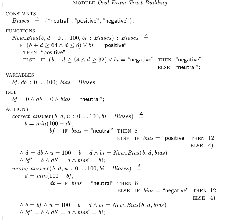
Fig. 1. State Transition System for Adapted Trust Building in Oral Exams
