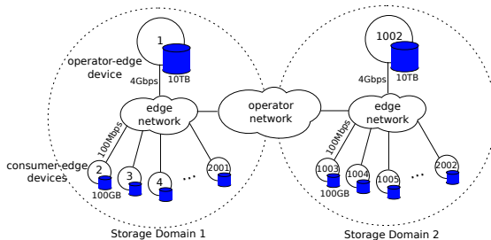
Fig. 3. Evaluation scenario
