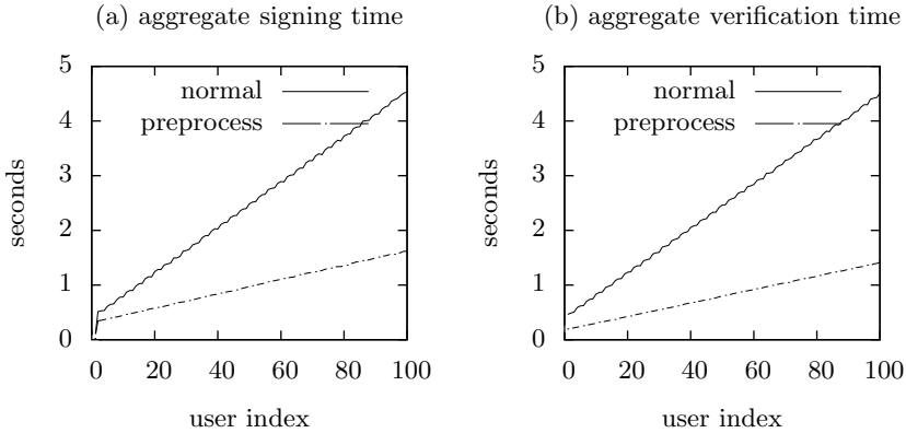
Fig. 1. Performance of our SAS scheme
