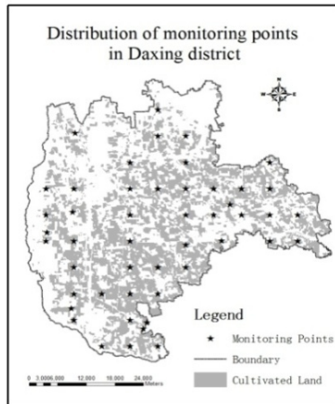
Fig. 5. Distribution of monitoring points in Daxing district
