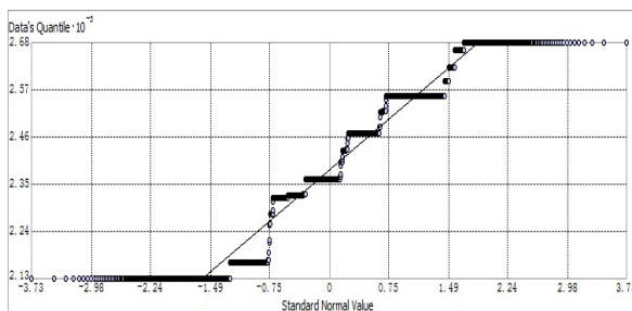
Fig. 2. Normal QQ Plot: the quantile values of the standard normal distribution are plotted on the x-axis, and the corresponding quantile values of the dataset are plotted on the y-axis
