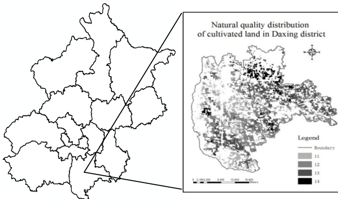
Fig. 1. Study area. Daxing district, located in the south of Beijing, has four natural quality grades (from 11 to 14), showing the ladder-like distribution from northeast to southwest. Higher quality land of 14th grade mainly in northeast makes up 7.72%, that of 13th grade 36.19%, that of 12th grade 35.35% and the rest mainly located in middle and south area belongs to 11th grade.
