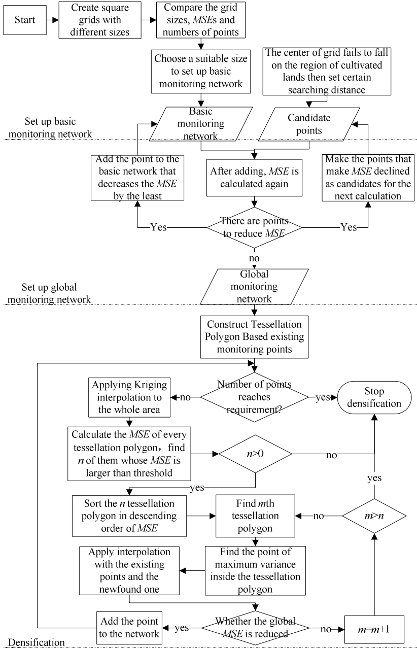
Fig. 3. Workflow of setting up the network: N could be set to the final count of samples according to the cost ( N=5182 by default). A threshold could be set and new points are added to n regions whose MSE s are bigger than the threshold ( n equals the number of global sampling points by default). Variable m is initially set to 1.
