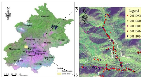
Fig. 1. The location of study areas and in-situ Measurements
