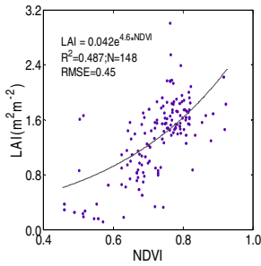
Fig. 3. Exponential model Between NDVI and LAI
