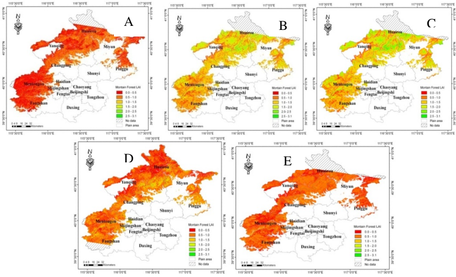
Fig. 6. Multitemporal Maps of retrieved forest LAI (A) Forest LAI map in April ; (B) Forest LAI map in June ; (C) Forest LAI map in August ; (D) Forest LAI map in September ; (E) Forest LAI map in October
