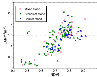
Fig. 8. The scatter of LAI and NDVI in different vegetation types
