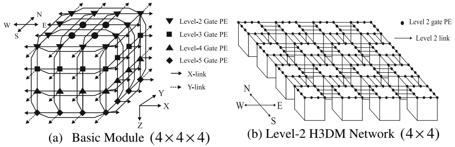
Fig. 1. Interconnection of a H3DM Network
