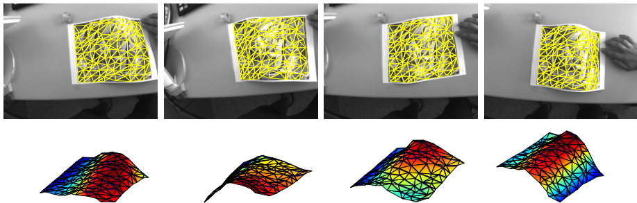
Fig. 3. Estimated structure for the strong deformation paper . Top: Deformed 3D mesh overlaid on the image sequence. Bottom: General view of the 3D deformable surface.
