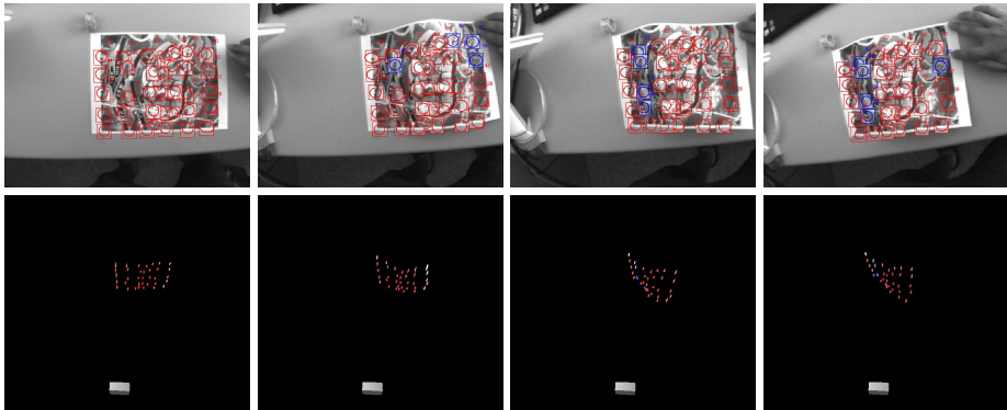
Fig. 4. Estimated structure for the strong deformation in real-time at 30Hz. Top: Images including elliptical search regions: red (predicted&matched) and blue (predicted&not matched). Bottom: General view of the 3D reconstructed deformed scene.
