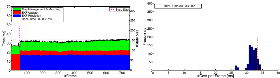
Fig. 5. Left: Real-time computation budget for the strong deformation sequence. Rigid initialization until frame#60 when non-rigid estimation starts. Two scale plots: left-y axis time, right y-axis state size n . Right: Per cycle time histogram.
