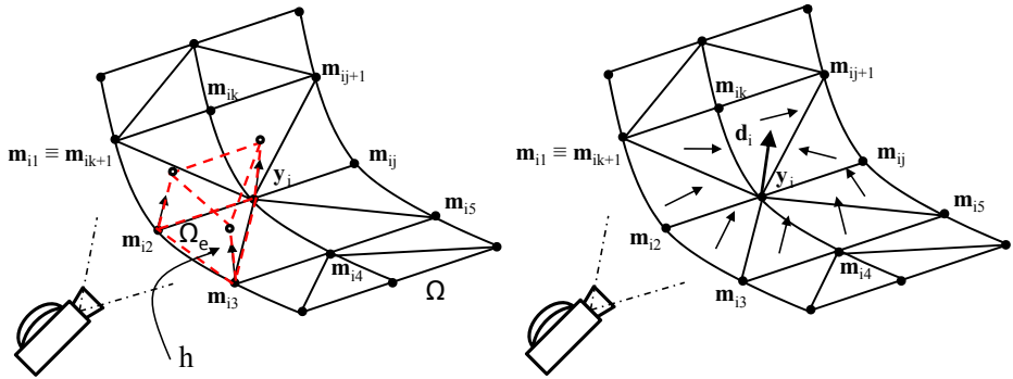
Fig. 1. Left: Extruded wedge element. Right: Extrusion normal unit vector \mathbf{d}_i , estimated as a weighted average of the normals of the mesh triangles having the considered node \mathbf{y}_i as a vertex.
