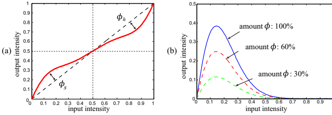
Fig. 6. (a) S-curve, \phi_s , \phi_h control the magnitude of S-curve adjustment in the shadow range and the highlight range respectively. (b) the curves of f_{\Delta}(x) weighted by different amount \phi .
