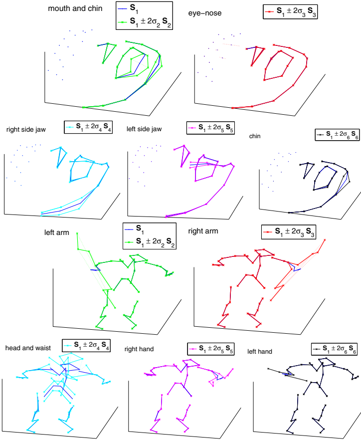
Fig. 4. The 3D shape bases obtained in the first 6 iterations of Algorithm 2 on face1 and stretch . The 3D basis shapes S_2, \dots, S_6 correspond to sub-shape deformations around the rigid shape component S_1 of the first iteration. These deformations are shown as S_1 \pm 2\sigma_i S_i , with \sigma_i the standard deviations of the corresponding coefficients. Note that the original motion capture markers on stretch were not located along straight lines.
