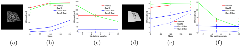
Fig. 4. Reconstructing a 2 \times 2 mesh from well- and poorly-textured images. (a) Sample well-textured input image. 3D error as a function of (b) the 2D input noise, and (c) the number of training examples. (d-f) Similar figures for the poorly-textured case. Note that our results are much more accurate than the baselines.
