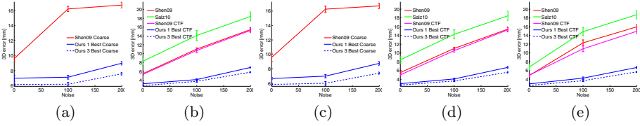
Fig. 5. Reconstructing a piece of cardboard from well-textured images. 3D error when (a) using a coarse ( 3 \times 3 ) mesh and no smoothness, and (b) refining the results of (a) with a gradient-based method. (c-d) Similar results as (a-b) but with smoothness. (e) 3D errors when manually increasing the influence of the smoothness term for refinement. Shen09 and Salz10 were directly obtained using a fine mesh. Note that our coarse results give a much better initialization for the refinement step.
