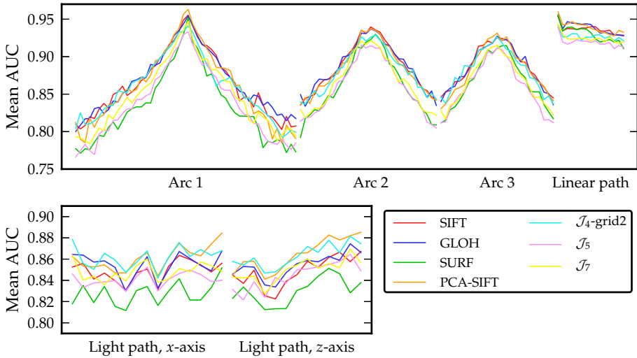
Fig. 3. Performance comparison with other state-of-the-art descriptors using MSER interest points
