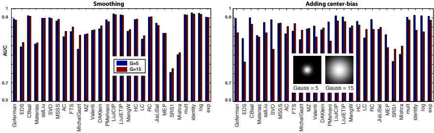
Fig. 8. Left: scores of models for maps smoothed with 2 Gaussian kernel sizes over ASD dataset. Right: model accuracy by adding Gaussian center-bias to center of a map.
