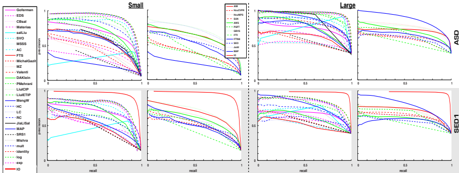
Fig. 4. Accuracy of models over small and large objects from ASD and SED1 datasets
