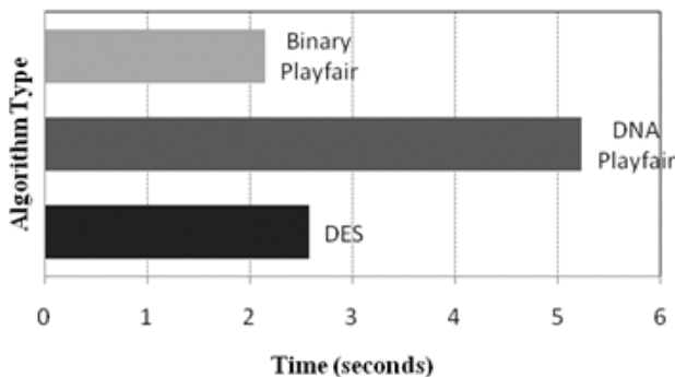
Fig. 4. Time requirement versus different encryption algorithms
