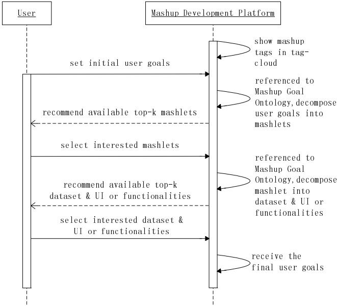
Fig. 3. Procedure of Goal Decomposition
