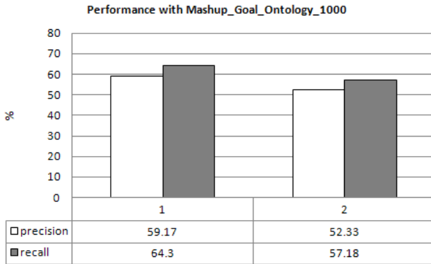
Fig. 6. Precision and Recall of Decomposition with Mashup_Goal_Ontology_1000
