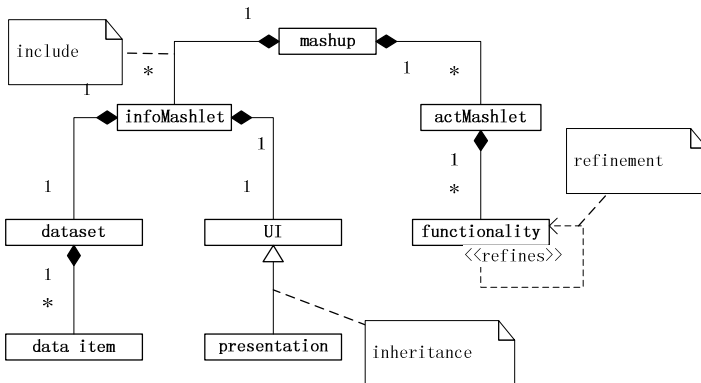
Fig. 2. Mashup Goal Ontology Model
