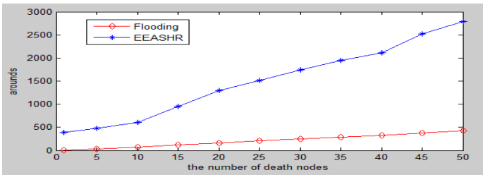
Fig. 3. network lifecycle of different protocol in the same initial energy
