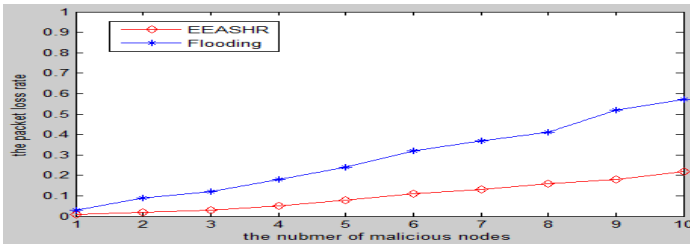
Fig. 4. network packet loss rate in different number of malicious nodes
