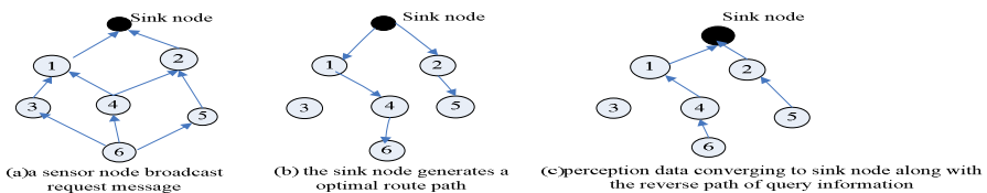
Fig. 2. The schematic plot for routing idea that No.3 is a malicious node
