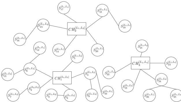
Fig. 1. Cluster-based multilevel security model example
