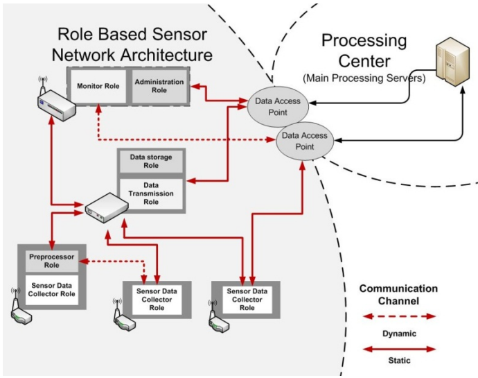
Fig. 1. Role Based Sensor Architecture Model
