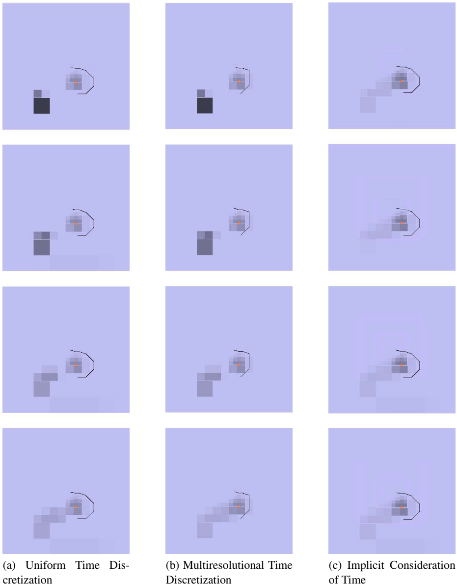
Fig. 4. The planning robot aims to reach a position behind the ball to dribble it to the goal. An opponent is detected and its position is propagated over the time by elongating the corresponding obstacle shape. At the beginning costs of cell nodes are calculated using a circular obstacle model. With increasing time, the obstacle representation becomes more elongated until it reaches the target, i. e. a position behind the ball opposing our target. The time increases from the top ( t=0 ) to the bottom images ( t=8 s). The left image series shows the uniform time discretization, the middle series the multiresolutional time discretization and the right series the implicit consideration of the time.
