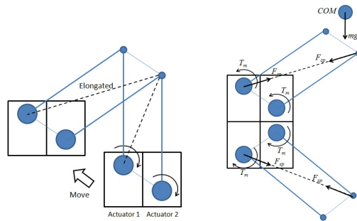
Fig. 6. Left: Concept of the spring assisted parallel four-bar linkage with synchronized actuation. Right: Diagram of CHARLI-L's leg.
