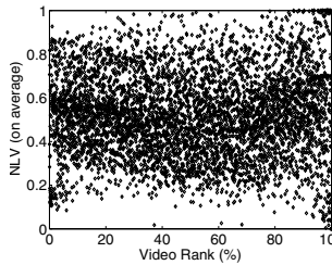
Fig. 5. NLV for videos of decreasing popularity. (100%: the least popular).
