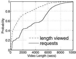
Fig. 1. Cumulative distribution of requests and viewing length of videos of different sizes
