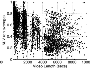
Fig. 2. Scatterplot of averaged NLV for each video of different lengths. One point per video.
