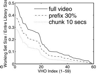
Fig. 6. Fraction of working set size to the entire library size at each VHO
