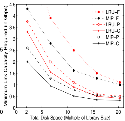
Fig. 9. Feasibility region of Placement-based and Caching-based solutions (the ordering of the curves is the same as in the legend)
