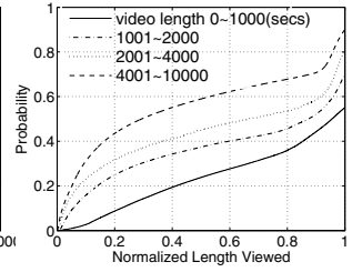
Fig. 3. Cumulative distribution of NLV for different classes of video lengths
