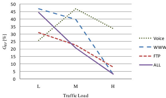
Fig. 5. RF EE gains for each simulated case
