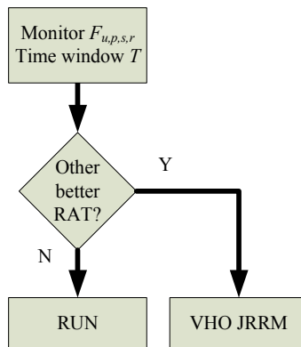
Fig. 4. The FF VHO triggering process (on-going connections)
