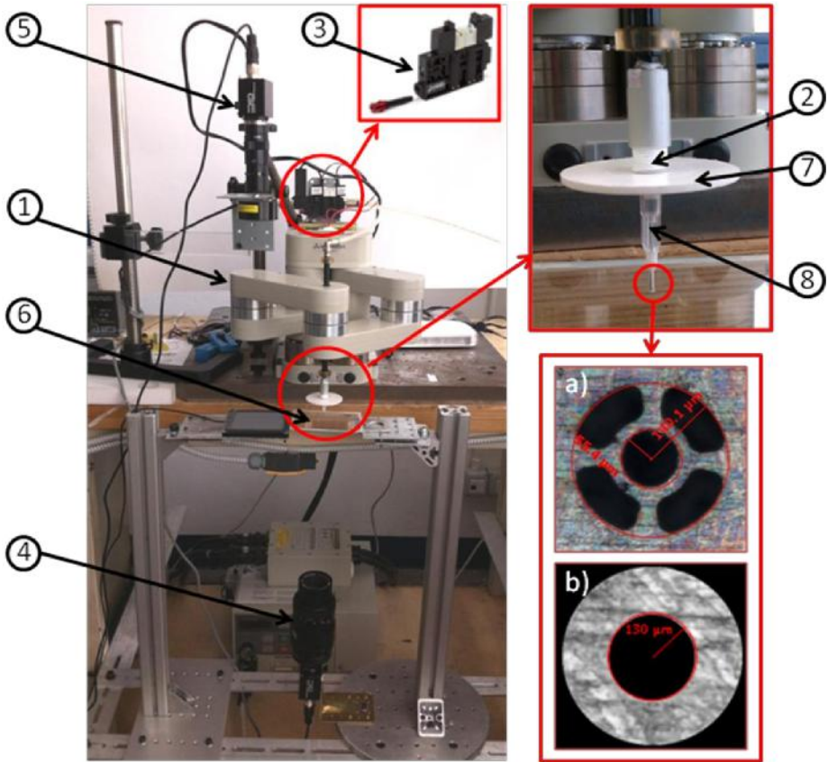
Fig. 1. Experimental setup
