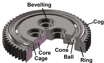
Fig. 1. Cutaway drawing of a ballbearing
