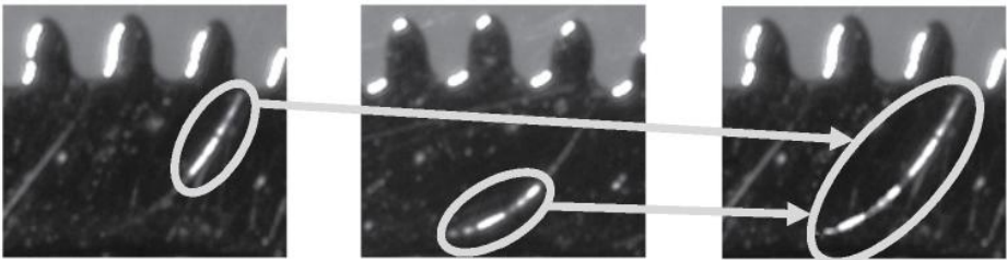
Fig. 10. The blobs of the same anomaly, which are detected on images acquired with different directional illumination, are combined together and processed jointly in order to extract features. The blobs from the two images are joined together by calculating the maximum between the pixels of the blob in one image and the pixels at the same locations in the other image. The result is shown in the image on the right.
