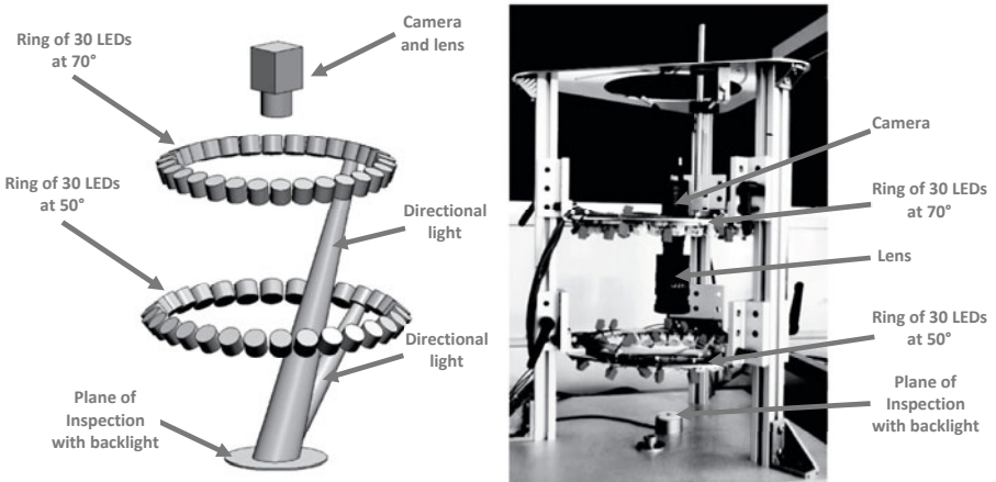
Fig. 6. Acquisition setup for the inspection of the ballbearings. The axis of the camera is perpendicular to the plane of inspection. The setup allows the use of different illuminations: backlight, ring light and direction alluminations at elevations of 50° and 70°.
