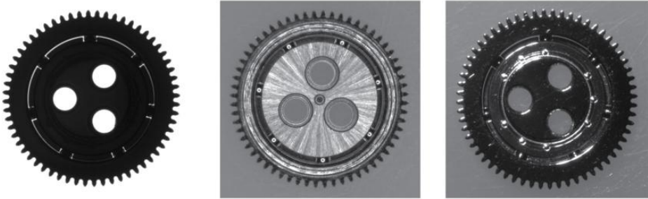
Fig. 7. Images of the ballbearing obtained using different illuminations: backlight (on the left), ringlight (at the center) and directional illumination (on the right).
