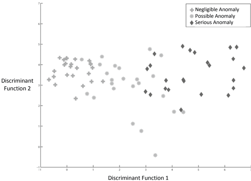
Fig. 11. Linear discriminant analysis applied to the features extracted from the anomalies detected on the surface of the ballbearing
