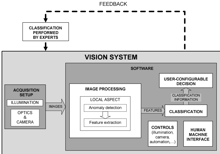
Fig. 5. Block diagram of the system
