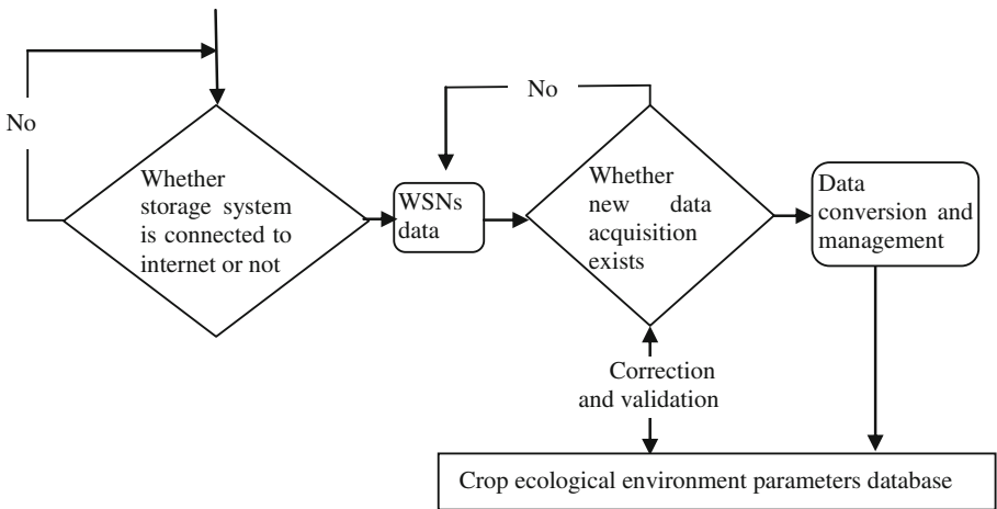
Fig. 3. Data reception conversion module scheme
