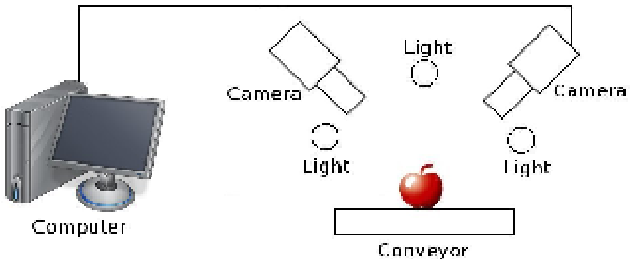
Fig. 4. The machine vision system
