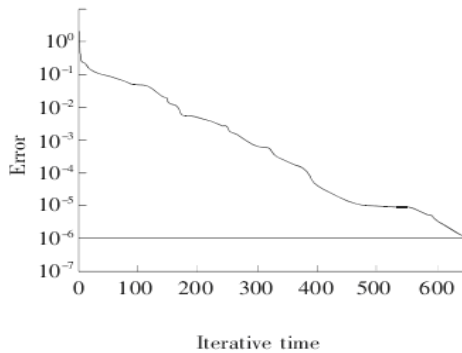
Fig. 5. Training result
