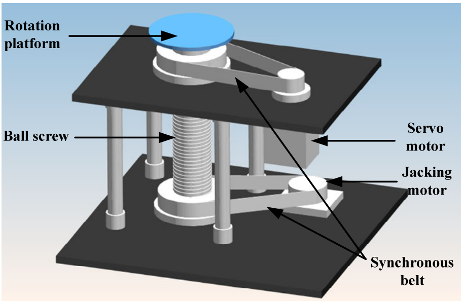
Fig. 2. Structure diagram of the jacking-rotation device
