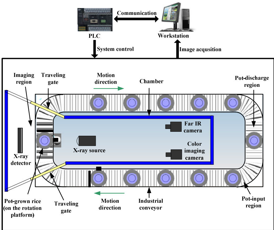
Fig. 1. Schematic drawing of the rice phenotyping automatic extraction system
