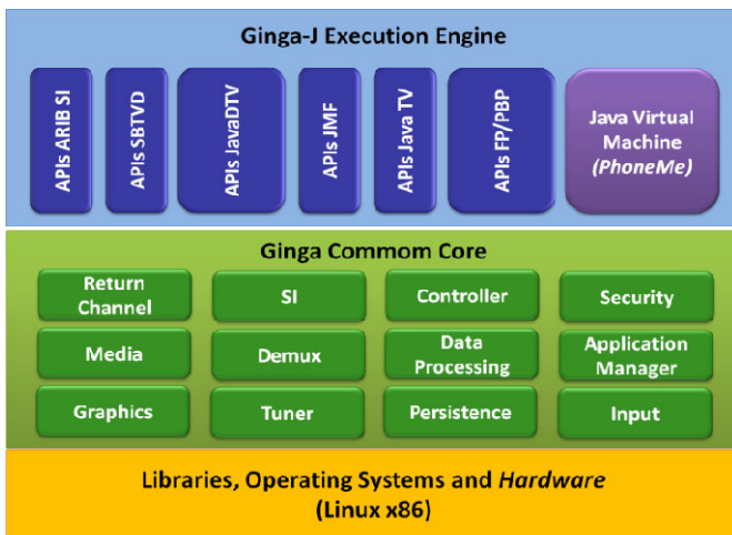
Fig. 4. Conceptual Architecture
