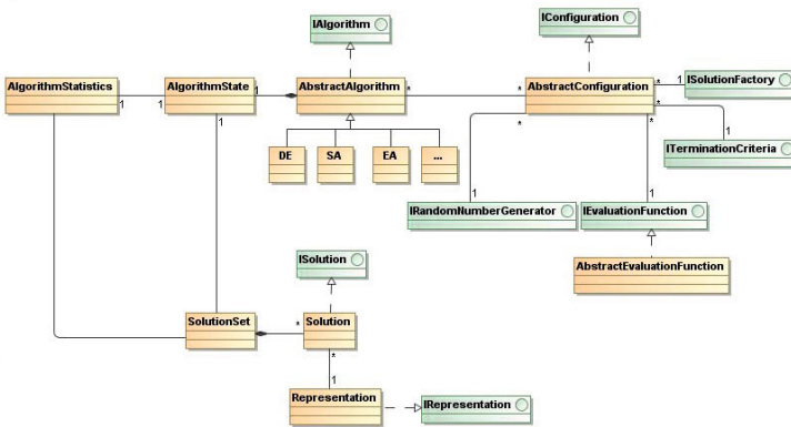
Fig. 1. Architecture of the JEColi: main classes
