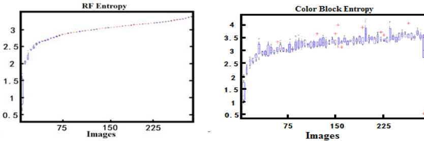
Fig. 2. RF-based entropy and block-based entropy
