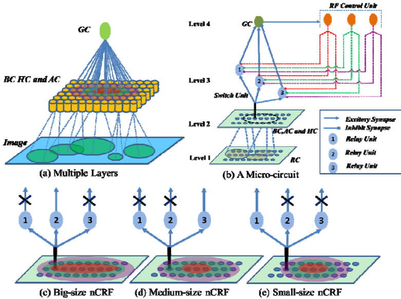
Fig. 1. A multi-layer neural architecture and how a GC adjusts its nCRF dynamically (a) is a multiple layers architecture. For the sake of clarity, only one GC and its nCRF is drawn. A nCRF has three rings with positive, negative and positive weight values. (b) This is a neural circuit of nCRF adjusting dynamically, which is a small function unit of (a) in detail. Because a neuron can change its output projection direction according to changing stimulus, nCRF can dynamically change its size. This can be realized by three relay neurons and three switch neurons. A switch neuron imposes its backward control on three relay neurons, and selectively permits only one relay outputting its signal upwards to GC. The relay neuron may have a chance to join one of three different rings of nCRF(c)-(d). With the different switch is turning on, the same neuron may exclusively participate in forming one of rings of a nCRF. Then a size-changing nCRF come into being. (c) is big one, (d) is middle one and (e) is small one.
