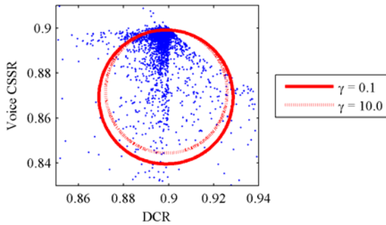
Fig. 3. Example of OC-SVM thresholds
