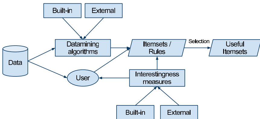
Fig. 1. MIME Workflow
