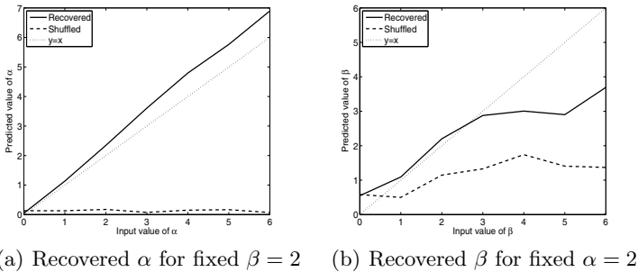
Fig. 8. Synthetic data. Recovering the peer coefficient \alpha and the authority coefficient \beta for the real data and the data after time-shuffle randomization.
