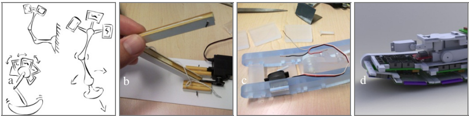
Fig. 1. Pictures of the iterative design process of Meerkat, some early sketches (a), cardboard exploration (b), acrylic exploration (c) and part of an exploded view in Solid Works (d)
