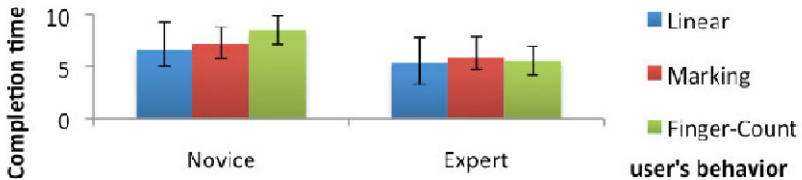
Fig. 5. Completion time by technique and user's behavior (95% confidence interval indicated)
