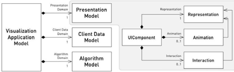
Fig. 4. Excerpt of Movisa’s metamodel, the relevant part for this paper is the Presentation Model , which defines UI components
