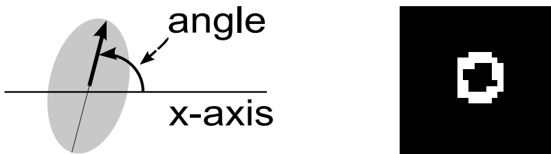
Fig. 4. Angle to x -axis ( left ). A circular contour ( right ).
