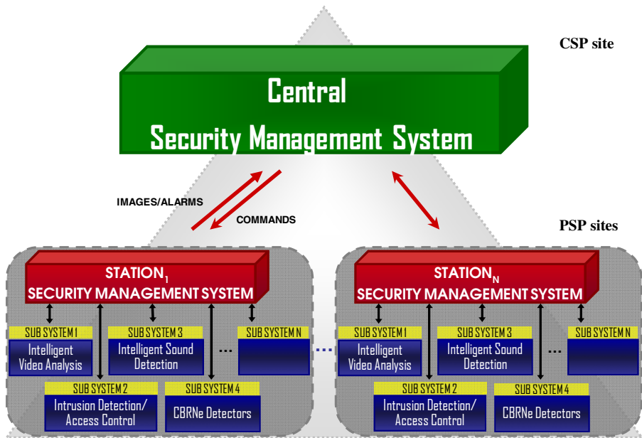
Fig. 1. SMS architecture
