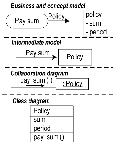
Fig. 5. An example of process and concept elements transformation into class elements
