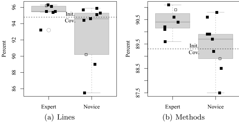
Fig. 2. Test Coverage
