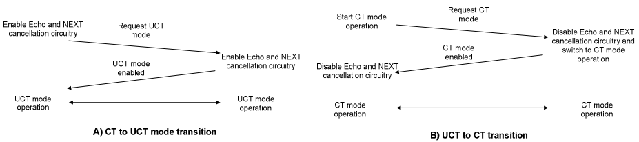
Fig. 5. Message exchanges to change mode of operation
