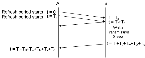
Fig. 4. Detailed transmission time diagram for the proposed scheme
