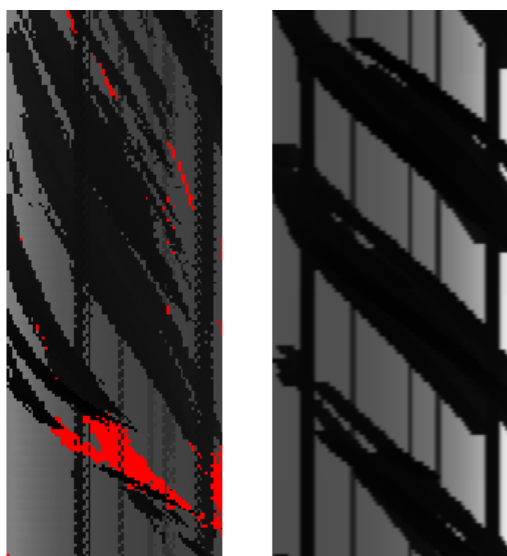
Fig. 10. Saturation and laser measurements as a function of time for the Sick LMS200. The vertical axis indicates time, the horizontal axis indicates measurement angle. Left real measurements from [11]. Right a reconstruction in simulation.
