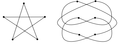
Fig. 1. C_5 and C_6 drawn as thrackles
