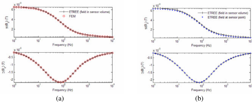
Fig. 2. Comparison of the magnetic field signal ( z -component) predicted by ETREE and FEM: (a) Case 1: ETREE considering sensor dimension vs. FEM; (b) Case 2: ETREE considering sensor dimension vs. ETREE predicting field at sensor point
