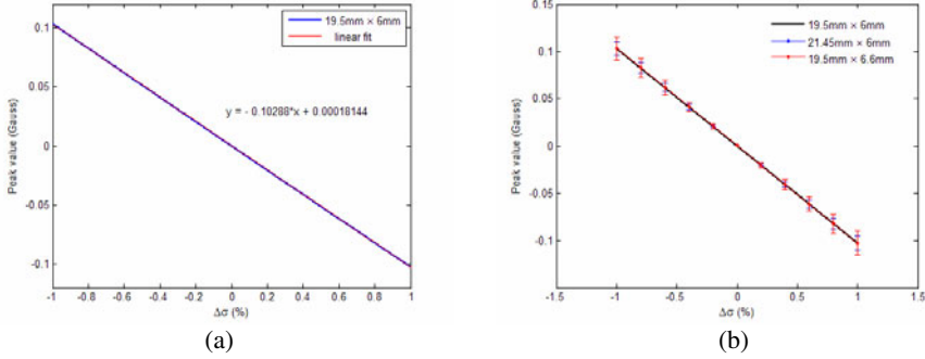
Fig. 3. PV against \Delta\sigma_i for (a) the coil ( x=19.5\text{mm} and y=6\text{mm} ) and (b) coils ( x=19.5\text{mm} and y=6\text{mm} ; x=21.45\text{mm} and y=6\text{mm} ; x=19.5\text{mm} and y=6.6\text{mm} )
