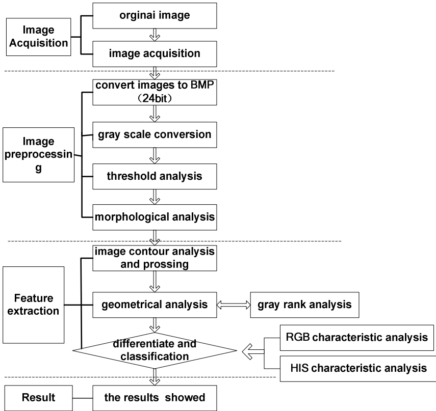
Fig. 2. Detection flowing chart of agricultural products' dimensions
