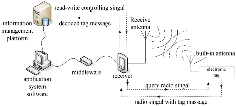
Fig. 3. Operation principle of RFID system
