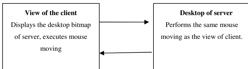
Fig. 3. How the client to control mouse actions of servers
