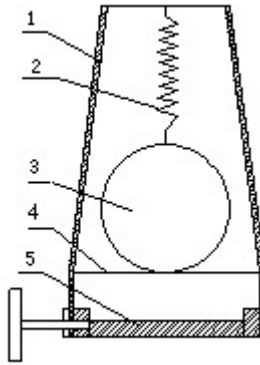
Fig. 1. Fixed water distribution device with round table 1-shell; 2-spring; 3-ball valve; 4-ball bar; 5-butterfly valve
