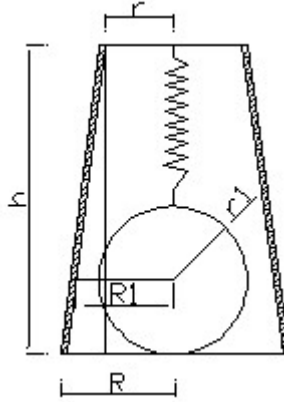
Fig. 2. Structure dimension of the device
