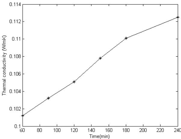
Fig. 4. Thermal conductivity of the frost layer
